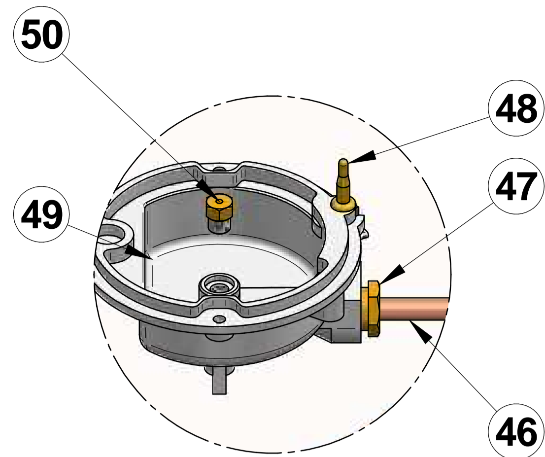
DETAIL A
